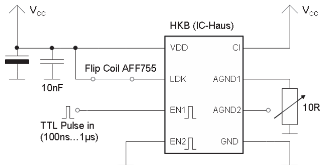
Fig. 8: Used laser diode driver circuit for generating short flip current pulses.
