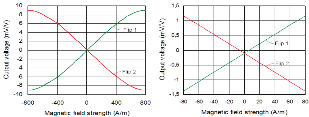
Fig. 1: Output voltage as a function of the magnetic field strength ( \alpha = 0^\circ ).
