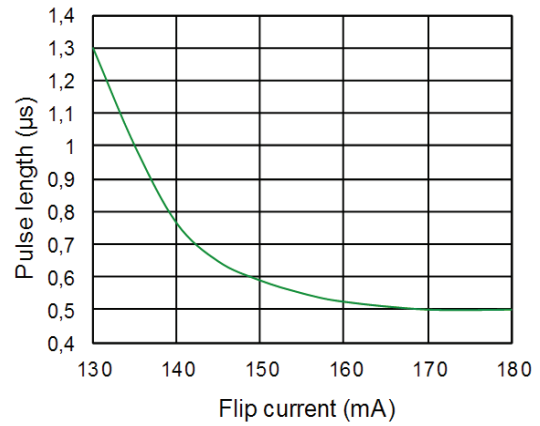
Fig. 7: Flip pulse length vs. flip current magnitude to achieve maximum resolution (see Fig. 10).
