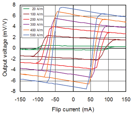
Fig. 2: Output voltage vs. flip current at different H_{ext} .
