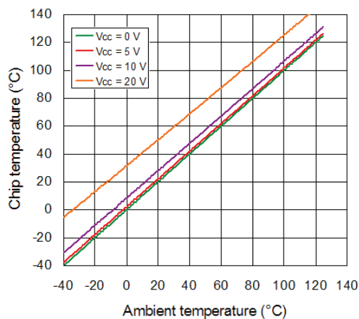
Fig. 10: Chip temperature vs. ambient temperature at different supply voltages.
