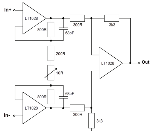
Fig. 9: Used instrumentation amplifier (Gain 100) for pre-amplifying sensor output signals.
