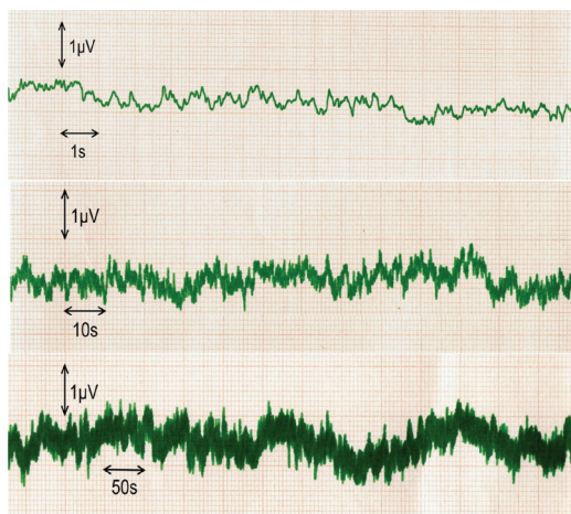
Fig. 4: Noise level for frequencies below 1 Hz ( V_{cc} = 5 V).
