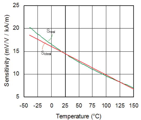
Fig. 3: Sensitivity vs. ambient temperature.
