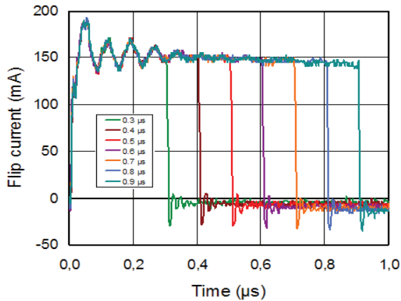
Fig. 6: Typically used flip pulses at different pulse durations (measured with Tektronix CT-1 Current Transducer).
