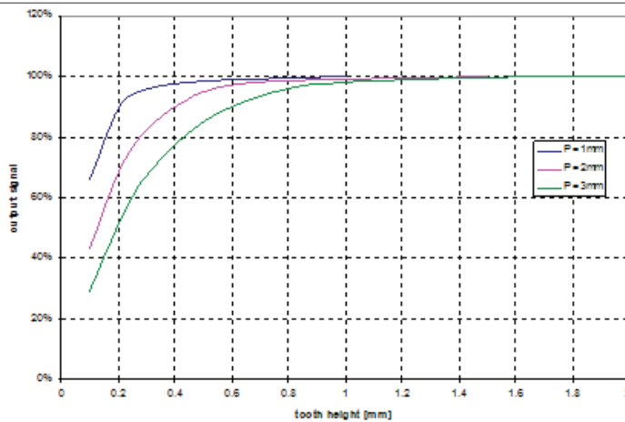
Fig. 7: Typical sensor output signal at a rectangular shaped tooth structure as a function of the tooth height.
