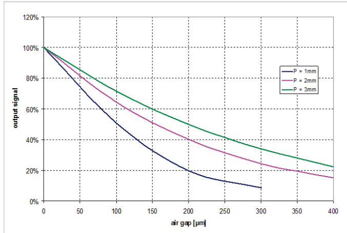
Fig. 6: Typical sensor output signal at a rectangular shaped tooth structure as a function of the air gap (distance between the sensor module and the tooth structure).
