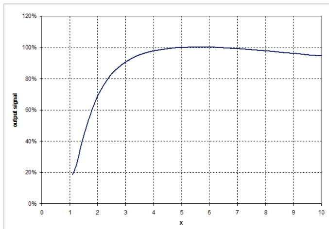
Fig. 8: Typical sensor output signal at a rectangular shaped tooth structure as a function of the land-pitch-factor x = P/w . P: pitch w: tooth top-land width
