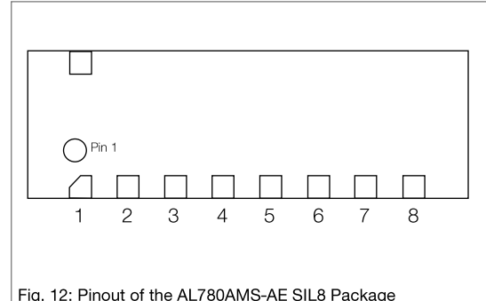
Fig. 12: Pinout of the AL780AMS-AE SIL8 Package
