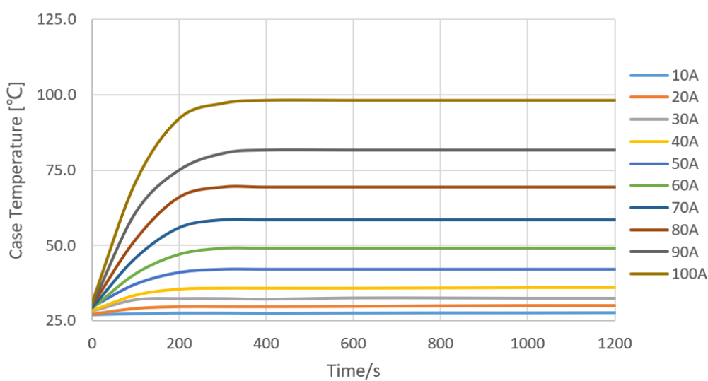
Figure 1. Relationship between STK-616AM5 Case temperature and amount of input current. Figure 1 shows the results of current & temperature measurement. Tested by using a standard demo test board, with 4 layers of copper conductors, where the thickness for each layer is 2 oz, the total thickness of demo board is 1.6 mm. This result is a reference data. Tc is changed much by the board layout and the heat dissipation. Please confirm it in your evaluation environment.
