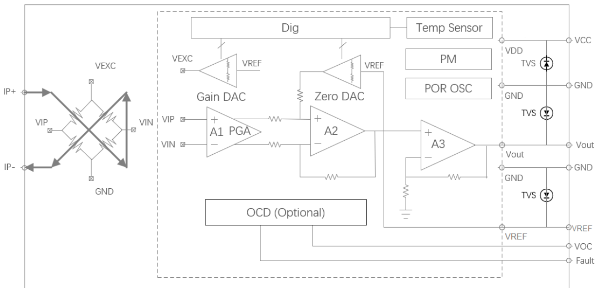
Figure 2 the functional block diagram for the STK-616TM series products.
