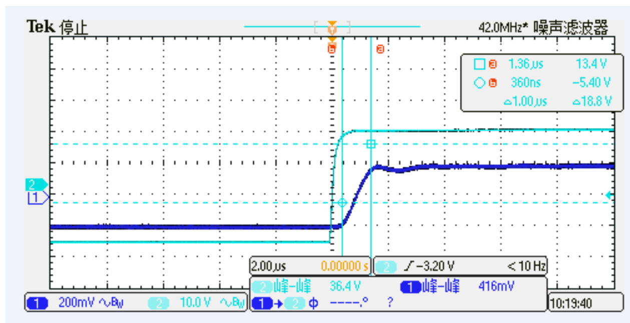
Fig.2 the step response time of STB-xxHA current sensors. The light blue is primary current, while the dark blue is output signal of current sensor. The step response time is less than 0.3 \mu s.
