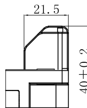
Detail-H 2:1
