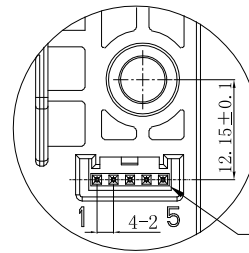
Detail-H 2:1
