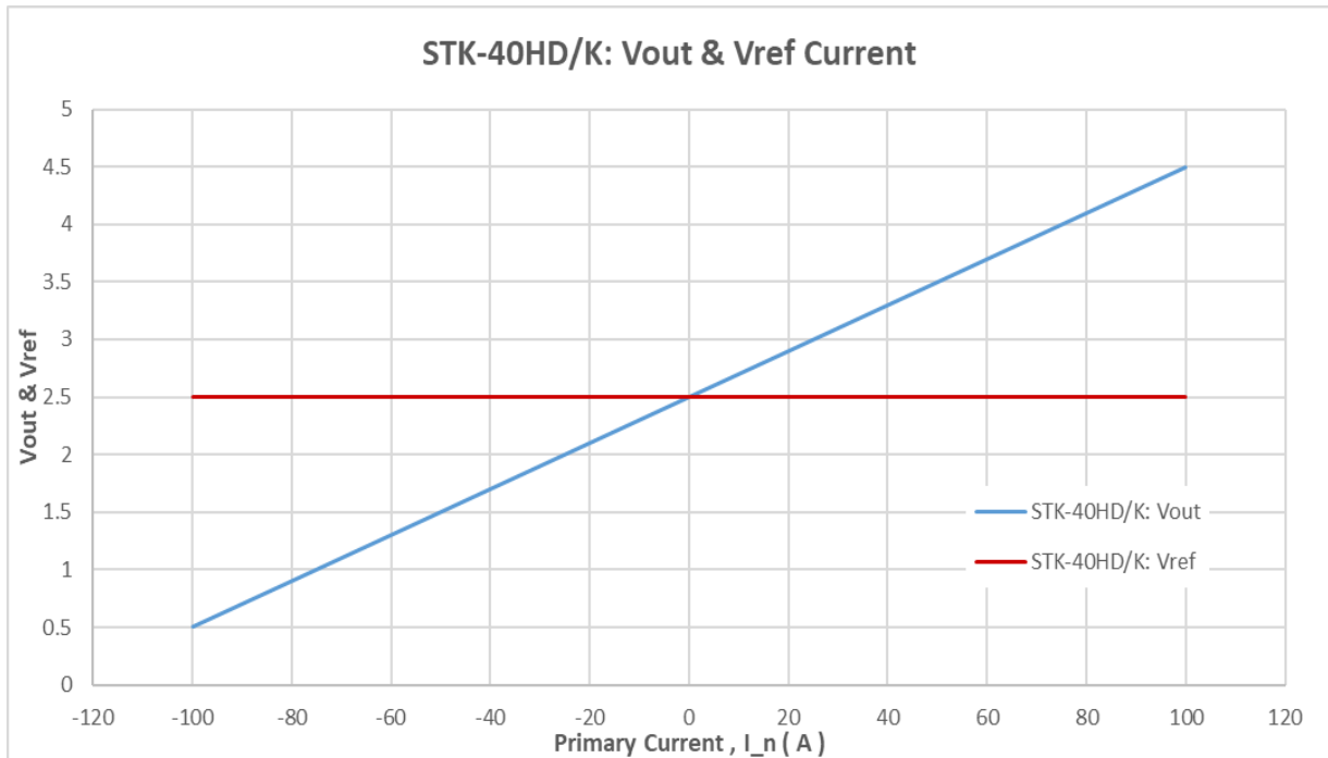
The dependence of Vout&Vref of STK-40HD/K on the primary current.
