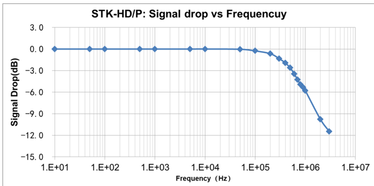
Fig.1 the frequency band width of STK-HD/P3 series current sensors.
