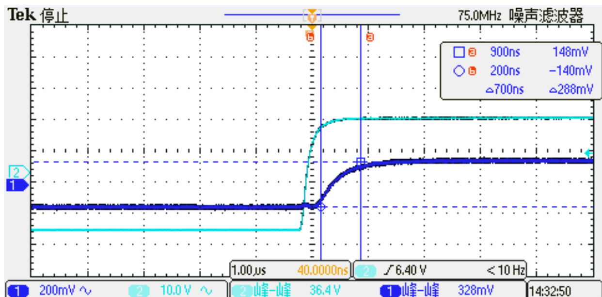
Fig.2 the step response time of STK-HD/P3 current sensors. The light blue is primary current, while the dark blue is output signal of current sensor. The step response time is less than 1.0 μs.
