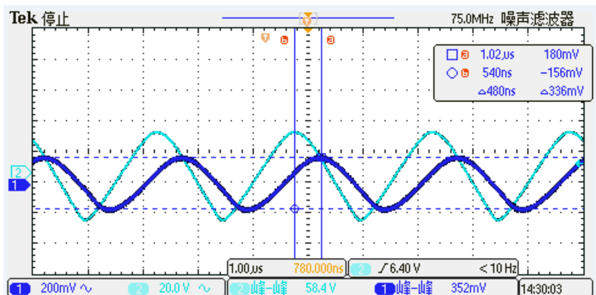
Fig.3 when detection the primary current with a frequency of 400 kHz. The delay time from the primary current (light blue) to the output of the sensor (dark blue) is around 0.5 \mu\text{s} .
